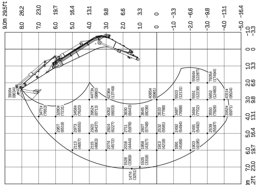
Over Side
